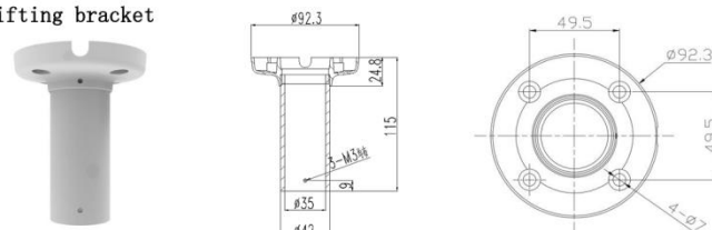
Lifting bracket
